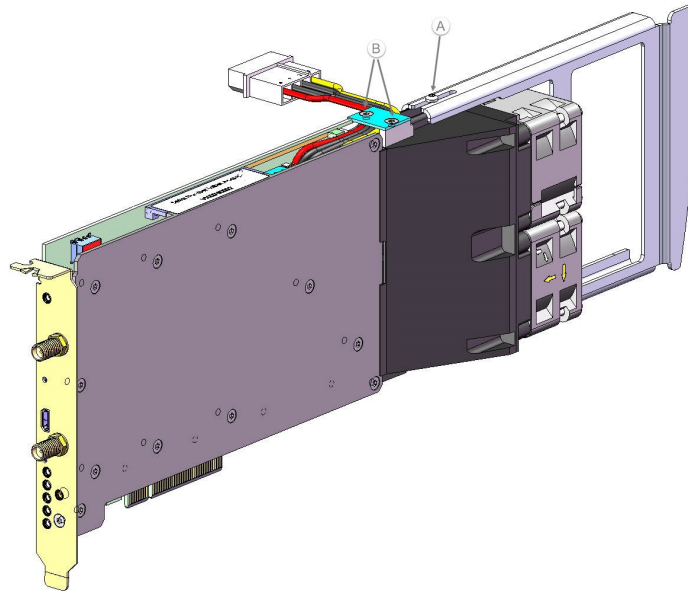
Diagram showing U5310A fan/support assembly fixings .
