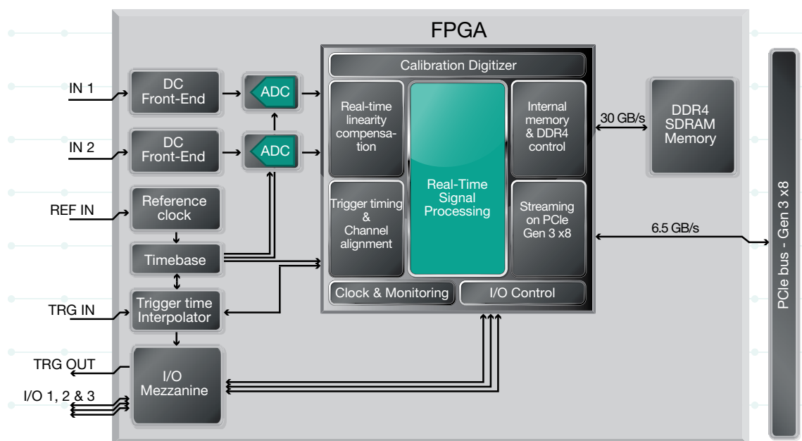
Figure 4. Top level block diagram of the SA240P PCIe ADC card, with on-board real-time processing.
